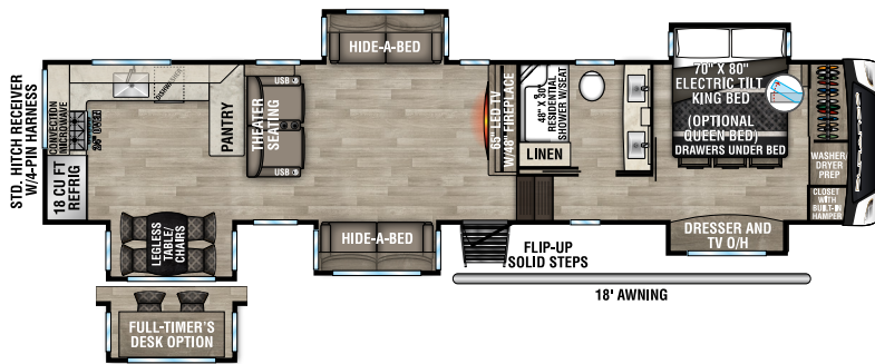
G391RKF UVV - 12,930 | Exterior Length - 42' 5" | Sleeps - 6
