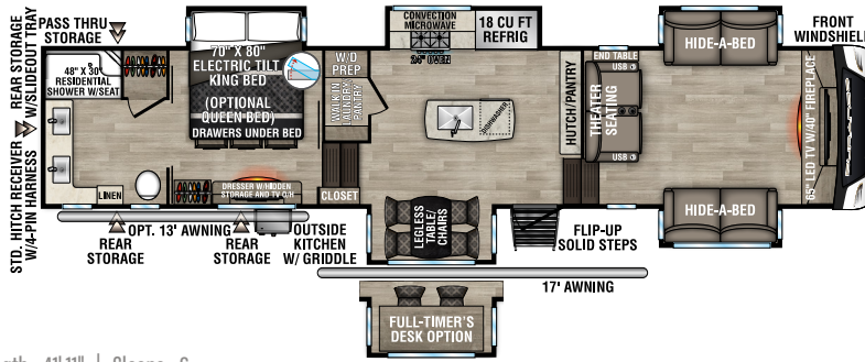
G387FLF UVV - 13,360 | Exterior Length - 41' 11" | Sleeps - 6
