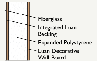
Wall Cut-Away
