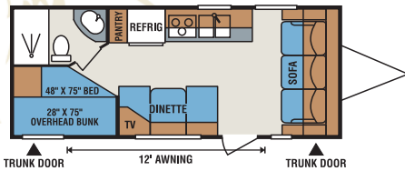
S221FL • UVW 3,690 • Dry Hitch Wt. 470 • NCC 1,310 • Length 23'11"
