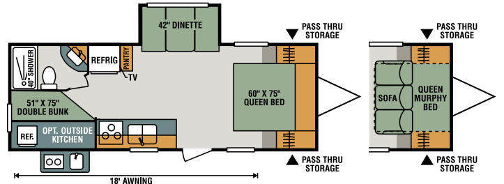
231BHLE Murphy Bed Option (patent pending)
