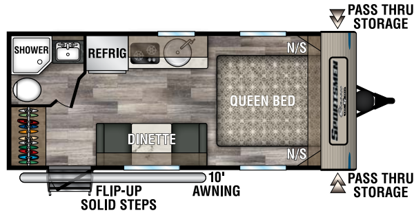
UVW - 2,860 | Exterior Length - 21' 10" | Sleeps 3
