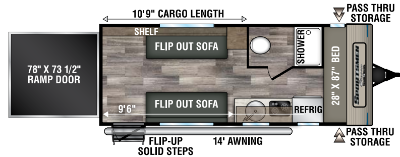
NEW 190TH UVW - 3,400 | Exterior Length - 22' 4" | Sleeps 3
