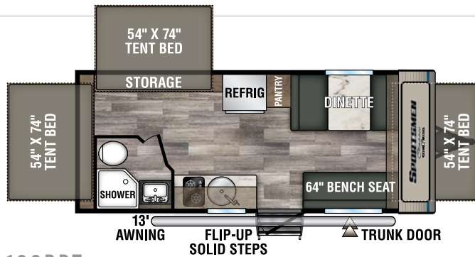
UVW - 3,250 | Exterior Length - 21' 6" | Sleeps 8
