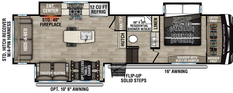
D301RLT UUV - 10,200 | Exterior Length - 34' 3" | Sleeps - 4
