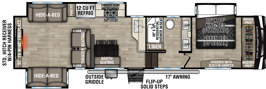
D326RLT UUV - 10,520 | Exterior Length - 37' 7" | Sleeps - 6
