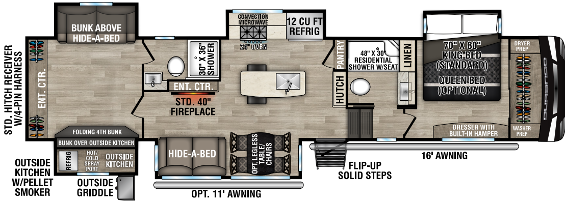
D348BHF UUV - 12,660 | Exterior Length - 42' 2" | Sleeps - 3
