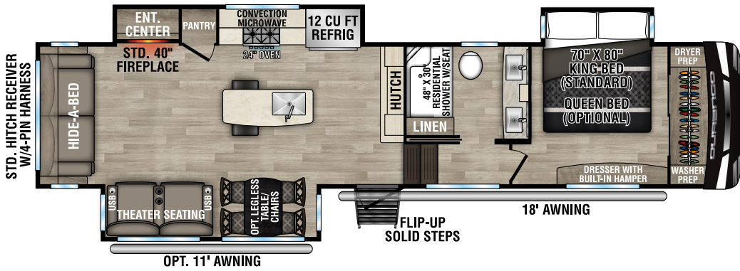
D333RLT UUV - 10,800 | Exterior Length - 37' 10" | Sleeps - 4
