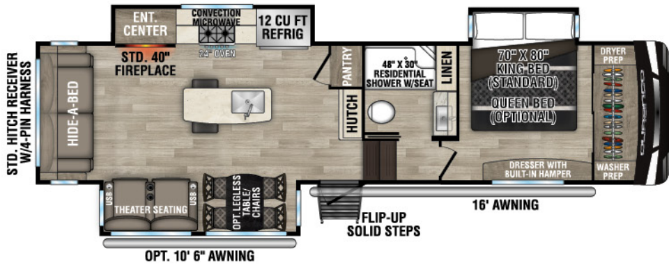
D301RLT UYW - 10,200 | Exterior Length - 34' 3" | Sleeps - 4
