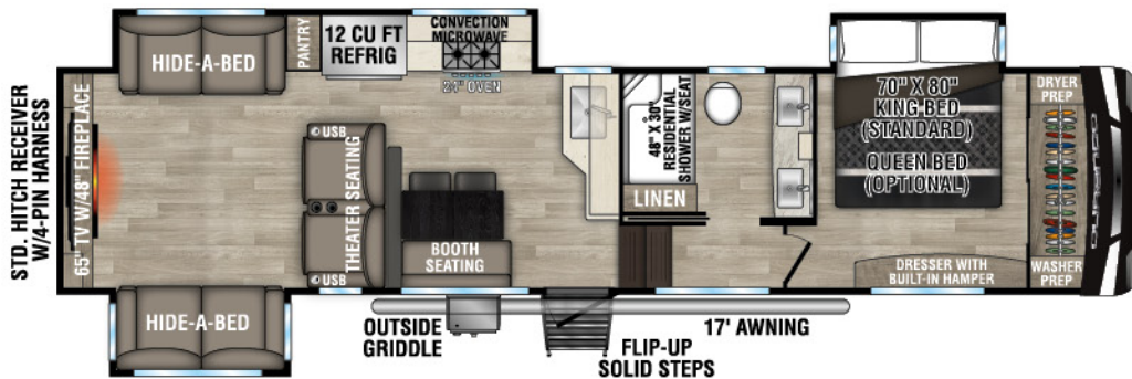
D326RLT UYW - 10,520 | Exterior Length - 37' 7" | Sleeps - 6
