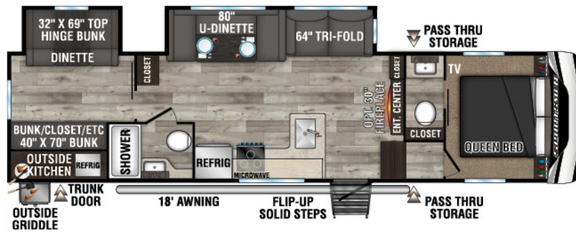
302BHK UWW - 8,680 Exterior Length - 35'9" Sleeps - 10
