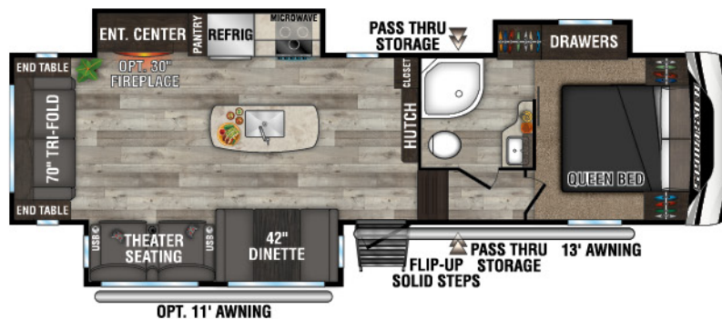
303RL UWW - 8,720 Exterior Length - 34'2" Sleeps - 5
